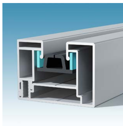
Fig. 4: Elaborate zip guide rail made from two separate plastic profiles. The outer one acts as a fastening rail and the inner one as a guide profile with coextruded spring elements.
