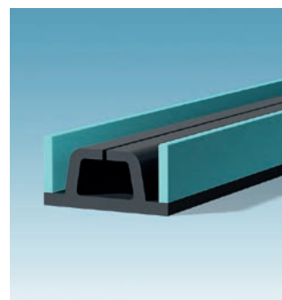
Fig. 2: In order to be able to guide the Zipscreens pulled tightly to the side, their reinforced outer edge features nubs made of a plastic with good sliding properties. They are guided in plastic profiles.
